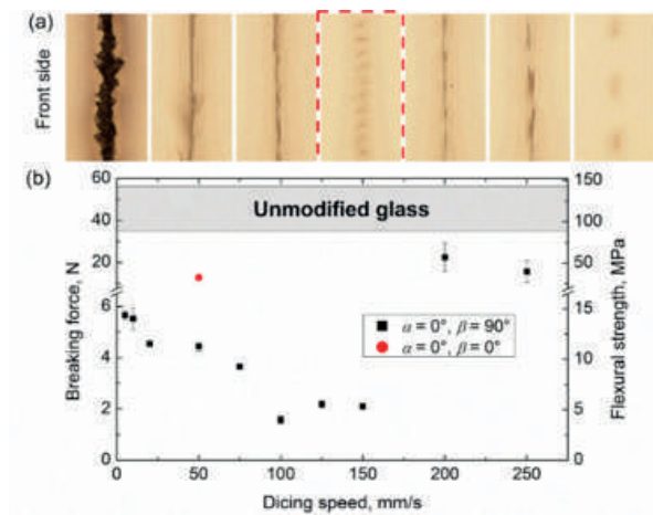
Fig. 4. (a) Optical microscope images of the front surface of diced samples with different speed and transverse cracks orientation, (b) bending force needed to fracture the Bessel beam modified glass as a function of dicing speed.
