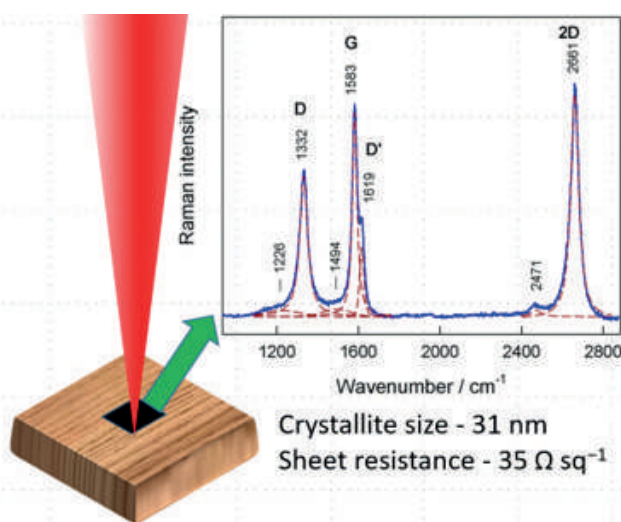
Fig. 6. Raman spectrum, corresponding crystallite size and minimal sheet resistance achieved with optimal 662 \text{ J/cm}^2 irradiation dose of nanosecond laser.
