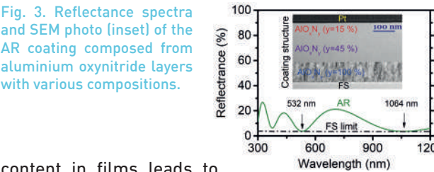
Fig. 3. Reflectance spectra and SEM photo (inset) of the AR coating composed from aluminium oxynitride layers with various compositions.
