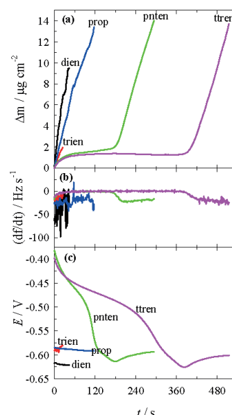
Fig. 1. Effect of amines on parameters of electroless cobalt plating process on a copper electrode: (a) change in mass gain, (b) frequency change rate and (c) open-circuit potential. Solution composition (mol l -1 ): amine – 0.005; DMAB – 0.2; CoSO 4 – 0.05; CH 3 COOH to pH = 5; 50 °C.
