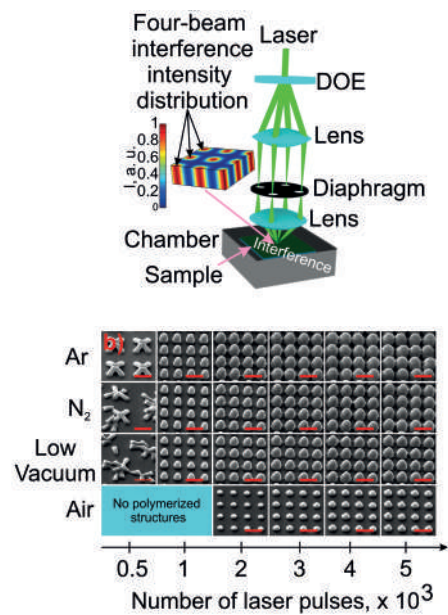
Fig. 4. (top) Experimental setup of four-beam interference lithography, (bottom) Morphology of the pillars fabricated in Ar, N_2 , low vacuum and air by using a different number of laser pulses (from 500 to 5000). Scale bars represent 10 \mu\text{m} .
