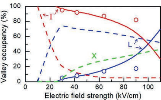
Fig. 5. The relative population of electrons in the \Gamma , L and X valleys of InAs as a function of the peak electric field. Monte Carlo simulation is represented by solid lines for 150 fs-long THz pulse, and by dashed lines for 0.8 ps-long pulse. The open circles are experimental data points.
