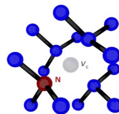
Fig. 1. The nitrogen-vacancy center in diamond.
