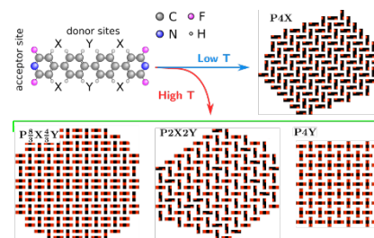
Fig. 4. (Top, left) BDFBPB molecule and (top, right and bottom) four self-assembled structures obtained by MC modeling. Black rectangle represents the molecule with differently damaged (red boxes) donor sites.
