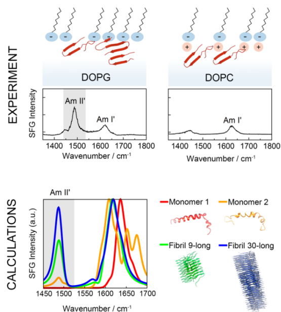
Fig. 1. (Top) Schematic representation of A \beta (1-42) aggregates adsorbed to DOPC and DOPG monolayers. (Bottom) Calculated VSFG spectra for various hypothetical A \beta (1-42) structures, indicating an increase of the amide-II' peak with increasing fibrillation.
