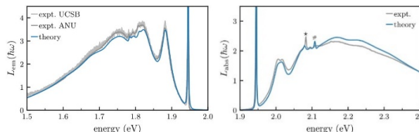
Fig. 2. Calculated (left) luminescence and (right) absorption lineshapes at nitrogen-vacancy centers in diamond (blue curves), compared to experimental ones (gray curves).
