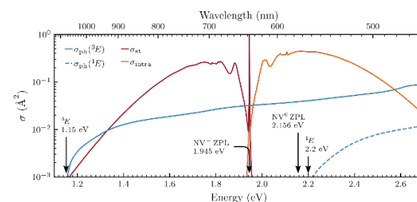
Fig. 3. Calculated photoionization cross section from the excited state 3E (blue curve), cross section for stimulated emission (dark red curve), and cross section for absorption (orange curve) for nitrogen-vacancy centers in diamond.
