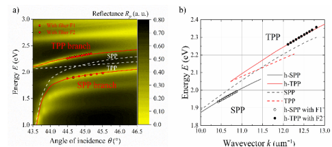
Fig. 11. (a) Dispersion of the hybrid TPP-SPP mode (red lines) with the calculated non-coupled single modes (yellow lines) and measured with filters (squares TPP branch and circles SPP branch). (b) Energy vs wavevector optical dispersion for the same sample.
