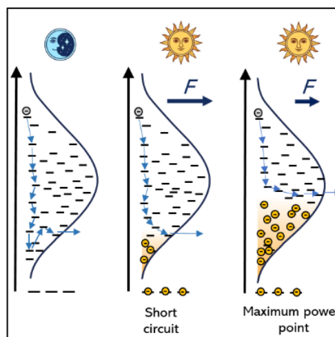
Fig. 1. Population of distributed density of states (DOS) and carrier relaxation within DOS at different solar cell operation conditions. The carrier mobility dynamics is determined by their relaxation within high energy part of the distributed density of states. The mobility strongly decreases with time independently of population of low-energy states.
