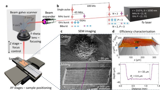
Fig. 1. Investigation of ultrafast laser burst-mode processing influence on ablation efficiency. (a) Principal scheme of laser processing setup. (b) Illustration of four possible laser working regimes: single-pulse, MHz burst, GHz burst, and biburst. (c) SEM images illustrate laser drilling and milling of copper samples and (d) corresponding graphs for efficiency evaluation.
