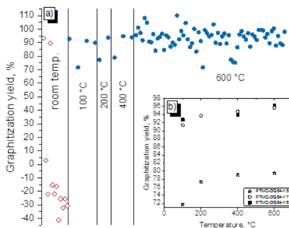
Fig. 4. (a) Graphitization yield of samples with a sulfur trap at temperature above 100°C (blue circles) and room temperature (red diamonds). (Inset) Graphitization yield of the three cremated bone samples at different temperatures.
