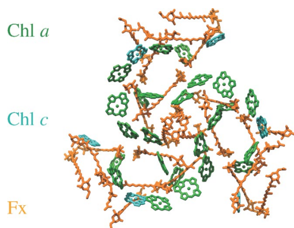
Fig. 2. Proposed pigment arrangement in the trimeric FCP of Cyclotella meneghiniana consistent with ultrafast spectroscopic data. Here Chl a/c is chlorophyll a/c and Fx is fucoxanthin. For clarity, Chls are only shown as porphyrins.
