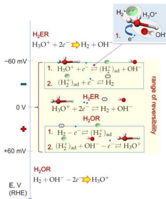
Fig. 4. Hydrogen evolution/oxidation reactions \text{H}_2\text{ER}/\text{H}_2\text{OR} in aqueous solutions. Inset: schematics of \text{H}_2^+ formation using pictorial of chemical structures of the participating species.
