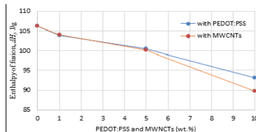
Fig. 2. The influence of shell modifiers PEDOT: PSS and MWCNTs on fusion enthalpy of paraffin PCM microcapsules.
