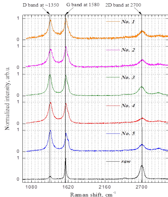
Fig. 1. The Raman spectra of graphite samples obtained from different locations of RBMK-1500 reactor. The excitation wavelength is 532 nm (0.3 mW).
