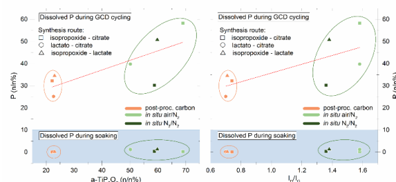
Fig. 2. ICP-OES determined phosphorus content in the electrolyte after soaking the electrodes in solution for ca. 24 h (blue area) or after 100 galvanostatic charge/discharge cycles at 1C rate (white area) with respect to (left) content of a-TiP 2 O 7 phase; (right) degree of structural disorder in carbon phase.
