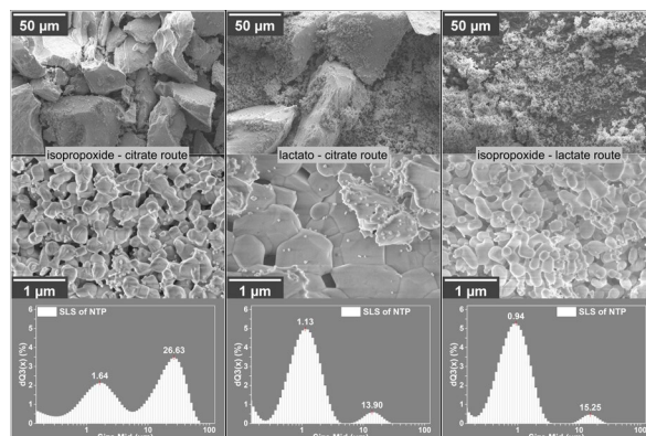
Fig. 1. SEM images and particle size distribution histograms (SLS) of carbon-free NTP materials derived by different sol-gel routes (isopropoxide-citrate, lactate-citrate, isopropoxide-lactate, respectively).
