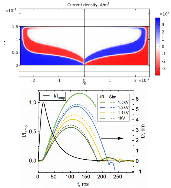
Fig. 4. (Top) Current density distribution within the superconducting armature after a magnetic field pulse. (Bottom) Trajectories of the superconducting armature and the driving current waveform.
