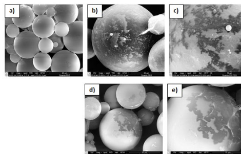
Fig. 1. SEM morphologic analysis of microcapsules MPCM32D: (a) unmodified, magnification 5000x; (b, c) with 5wt.% MWCNTs shell-modified, magnification 5000x and 10000x; (d, e) with 5wt.% PEDOT: PSS shell-modified, magnification 5000x and 10000x.
