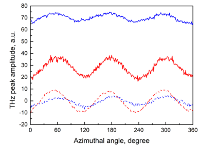
Fig. 7. Azimuthal angle dependences of THz emission from two samples: VS001 (blue) and VS002 (red). The spectra were measured in the transmission geometry: \theta=30^\circ (full lines) and \theta=0^\circ (dashed lines).
