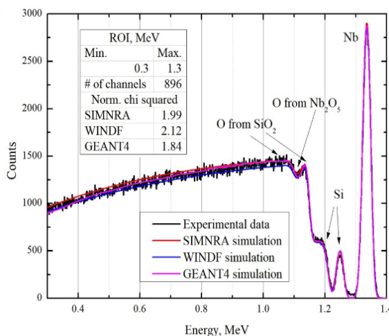
Fig. 5. Experimental and calculated spectra of proton RBS from SiO 2 /Nb 2 O 5 /SiO 2 sample.
