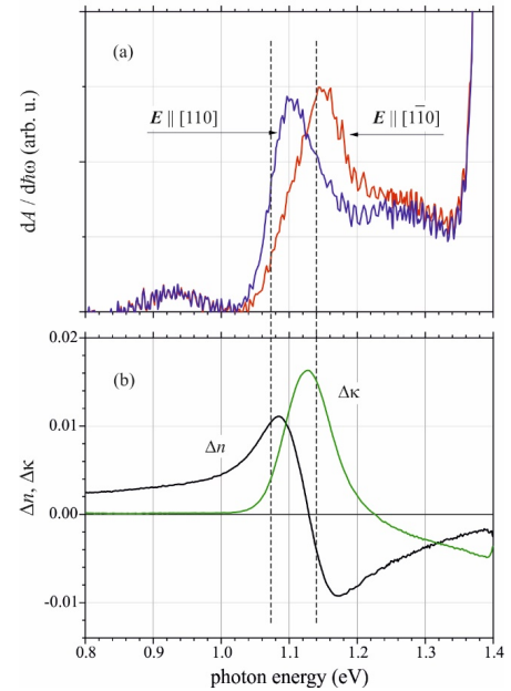
Fig. 11. (a) Optical density differential spectra and (b) the spectra of birefringence \Delta n = n_{[110]} - n_{[1\bar{1}0]} and linear dichroism \Delta \kappa = \kappa_{[110]} - \kappa_{[1\bar{1}0]} for the GaAs 1-x Bi x ( x=0.042 ) sample. Vertical dashed lines indicate spectral positions of the optical features observed in photo-modulated transmittance / reflectance spectra.
