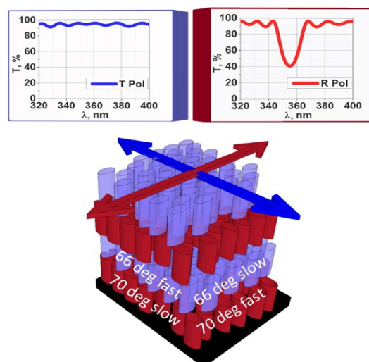
Fig. 15. The principal scheme of cross-sections of polariser for normal incidence angle, based on multi-layer coating consisting of anisotropic layers with perpendicularly aligned optical axes.
