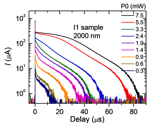
Fig. 10. Temporal response (photocurrent relaxation curves) of GeSn IR photodiodes (I1 sample) under 0.5 V reverse bias using different laser power at wavelength of 2000 nm. With the excitation increase, the response of the photodiode becomes slower due to the screening of charge separation potential by injected carriers.
