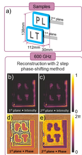
Fig. 1. Two 2D objects reconstruction at 600 GHz frequency using the phase shifting technique and Angular Spectrum of Plane Waves propagation method.
