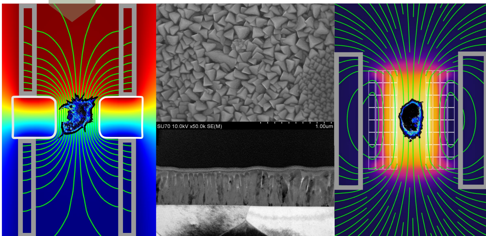
(Left) Electric field distribution in cross-flow treatment chamber during cell electroporation. (Right) Magnetic field distribution in pulsed coil magnet. (Middle) Electron scanning microscopy and transmission electron microscopy images of magnetoresistive La-Sr-Mn-O nanostructured film.
