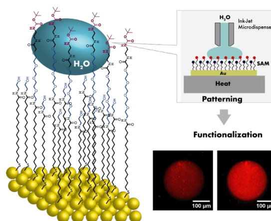
Fig. 1. Schematic representation of the self-assembled monolayer, micro-dispensing of water droplets and functionalization of the surface with quantum dots.
