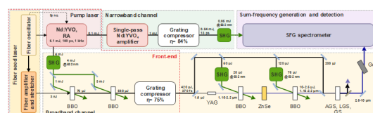
Fig. 7. The layout of the assembled SFG spectrometer setup.
