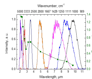
Fig. 8. The LGS OPA idler wave output spectra and pulse energies in the wavelength tuning range of 2 - 9.6 \mu\text{m} .
