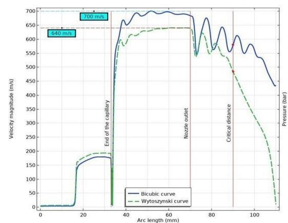
Fig. 18. Comparison of the velocity of Bicubic and Witoszynski curve nozzles.
