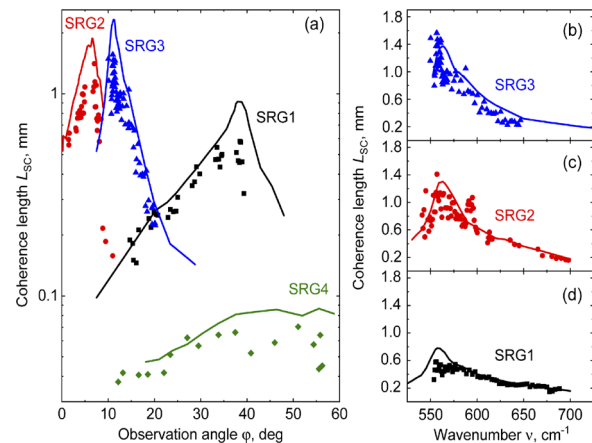
Fig. 9. (a) Coherence length dependence on the observation angle of the of SPPPhPs emission from four different n -GaN gratings SRG1, SRG2, SRG3, SRG4 with the period of 11, 16, 22, and 8 \mu\text{m} , respectively. Symbols denote the experiment and solid lines represent the RCWA calculations taking into account that angular field of view (AFO) is 0 deg. (b)–(d) Coherence length dependence on frequency of SPPPhPs emission from indicated samples. Symbols denote the experiment and solid lines represent the RCWA calculations taking into account that AFO=0.6 deg. Note that maximum of the coherence length is found in the vicinity of TO phonon frequency for all SRG samples.
