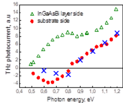
Fig. 4. The THz excitation spectra measured after InGaAsBi/InP structure excitation by femtosecond optical pulses from the layer and from the substrate side. Blue crosses are the results of the Monte Carlo simulation.
