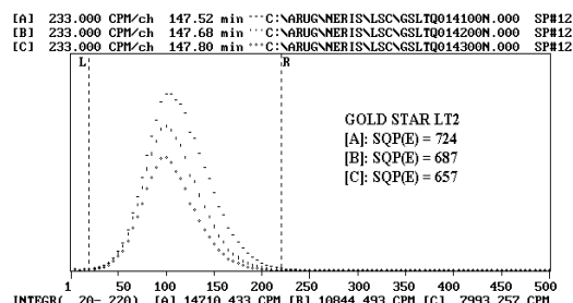
Fig. 1. Effect of quenching for the LSC cocktail (GSLT) at the sample-to-cocktail ratio of 10:10 mL. The spectra [B] and [C] are measured with added 20 and 40 \mu\text{L} of quenching agent, respectively. The SQP(E)=724 refers to the typical sample prepared with the GSLT cocktail.
