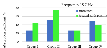
Fig. 3. Absorption ability of tested samples at 18 GHz frequency.
