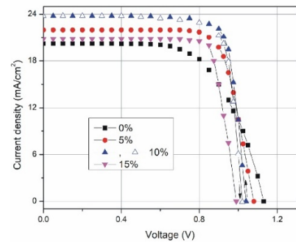
Fig. 6. Current voltage characteristics of perovskite SCs with different cesium concentrations.
