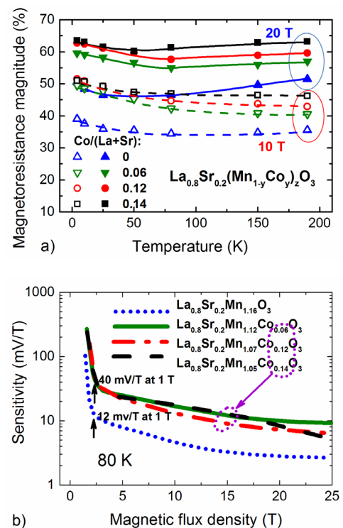
Fig. 5. (a) Temperature dependences of MR and (b) sensitivity dependences on magnetic flux density for La-Sr-Mn-Co-O films with different Co content.
