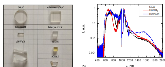
Fig. 5. (a) Materials tested for SC generation. (b) SC spectra of Raman active crystals.
