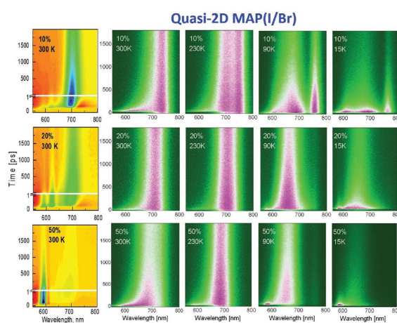
Fig. 4. Evolution of the transient absorption spectra at room temperature and evolutions of photoluminescence spectra at different temperatures measured for quasi-2D MAPI2Br1 samples with 10 %, 20 % and 50 % of butylammonium (BA) substituting MA.
