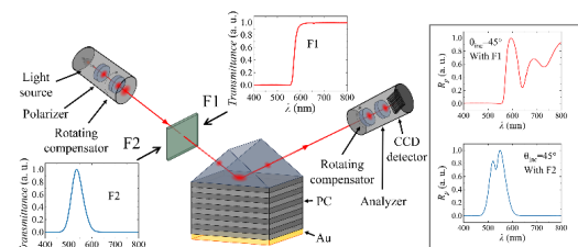
Fig. 10. Filters F1 (red line) and F2 (blue line). The optical response of the hybrid TPP-SPP mode is shown in graphs on the right side (top), h-SPP and h-TPP (bottom).
