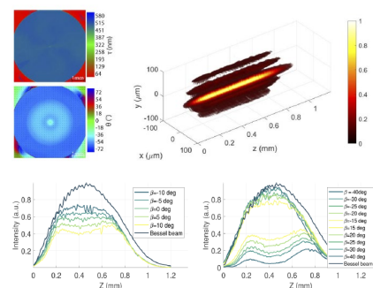
Fig. 2. Distribution of the retardance \tau and the slow axis \theta in the PBP element manufactured by Altechna R&D. (Top) The 3D intensity distribution in the optical needle created by the combination of the PBP element, the linear polarizer and the axicon. (Bottom) Distortions in the optical needle caused by the azimuthal misalignment between the polarizer and the PBP element for various values of the mismatch angle \delta .
