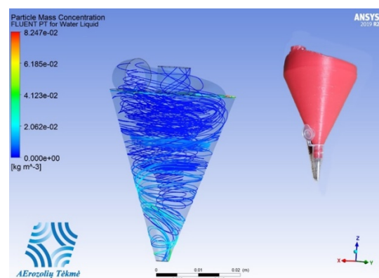
Fig. 7. (Right) Early working ‘Aerosol whistle’ prototype. (Center) Simulation of cyclonic airflow by computational fluid dynamics method.
