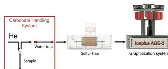
Fig. 3. Schematic view of graphitization line of cremated bones at Mass Spectrometry Laboratory.
