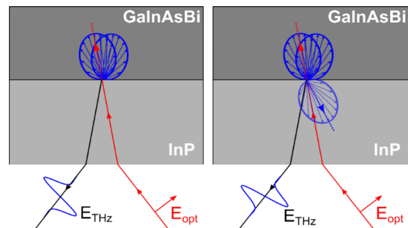
Fig. 5. The momenta of electrons excited from the heavy hole subband in the narrow bandgap part of heterostructure by linearly polarized femtosecond light pulse. (Left) The electron excess energy lower than the conduction band offset; (right) higher than the offset.
