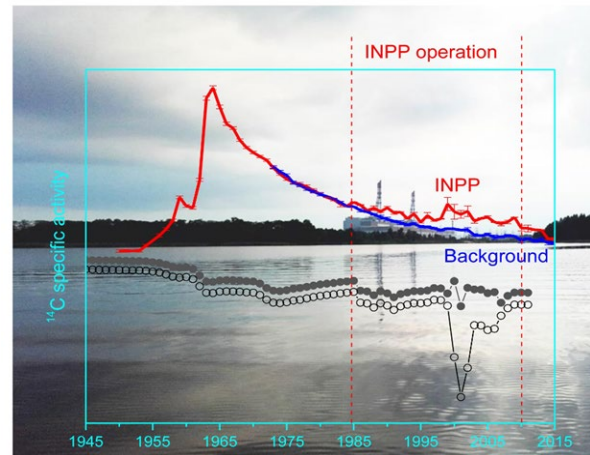
Fig. 6. Measured and calculated values of ^{14}\text{C} specific activity in the alkali-soluble and alkali-insoluble sediment fractions.
