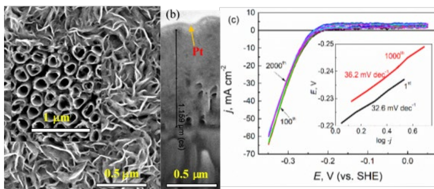
Fig. 5. (a) Top-side and (b) cross-sectional SEM images of hybrid \text{MoS}_2/\text{cyst} film whereas (c) depicts the CV plots in 0.5 \text{ M H}_2\text{SO}_4 solution up to 2000 potential scans. Insets: in (a) support SEM view, in (c) Tafel slope for indicated scan.
