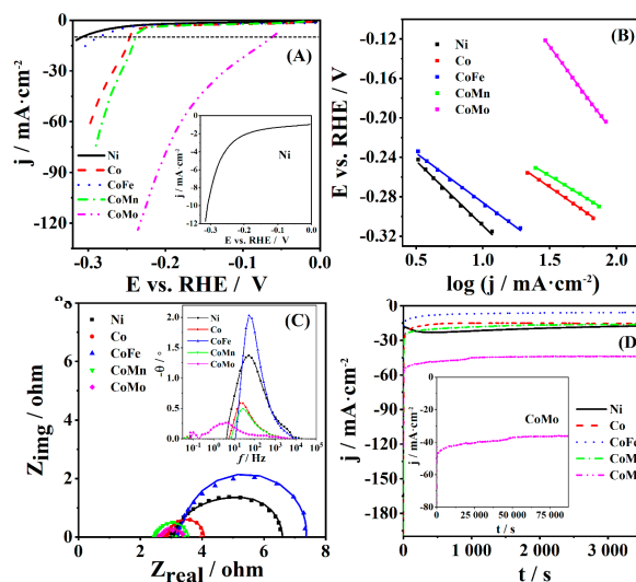
Fig. 1. (A) HER polarization curves (iR-corrected) of five studied coatings at 5 \text{ mV s}^{-1} with (B) corresponding Tafel plots. (C) Nyquist plots at -0.33 \text{ V} (amplitude of 5 \text{ mV} in the 100 \text{ kHz} – 0.1 \text{ Hz} range) with the corresponding Bode plots in the inset. (D) Chronoamperometric curves at -0.24 \text{ V} for 1 \text{ h} with the chronoamperometric curve of CoMo at the same potential for 24 \text{ h} (inset). All measurements were performed in 1 \text{ M KOH} .
