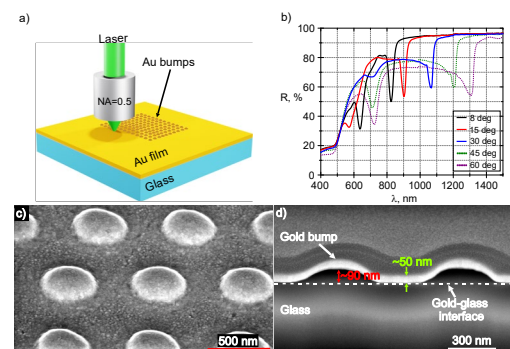
Fig. 2. (a) Illustration of Au bumps formation in a thin gold film using direct laser writing technique; (b) reflectance spectra of microbumps array with period 700 nm in 50 nm thick gold film at a different angle of incidence for p -polarized light; (c) SEM micrograph of fabricated gold bumps array in a thin gold film (50 nm); (d) cross-section of gold bumps.
