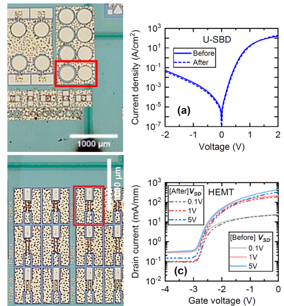
Fig. 8. Microscope images of the transparent SiC wafer with AlGaIn/GaN heterostructures and electronic devices being in a focus and laser ablated trenches being on the back side. Red colour rectangles indicate selected devices for investigations: Schottky barrier diodes (top left) and HEMTs (bottom left) and their corresponding current-voltage (I-V) characteristics on the right hand side. The same devices were characterized before (solid lines) and after (dashed lines) laser processing of trenches on the SiC wafer side in a depth up to 270 \mu\text{m} .
