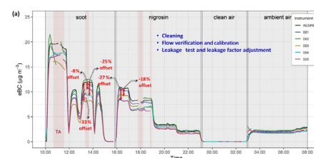
Fig. 3. Time-series of eBC mass concentrations at 880 nm.
