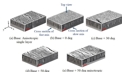
Fig. 14. The 3D representation of SEM images combination of (a) single layer with 250 nm thickness, deposited at an angle of 70° and 2-layers structures with the second layer deposited at (b) 0°, (c) 30°, (d) 50° and (e) 50° -anisotropic case. The red bar is set at 250 nm.
