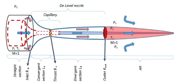
Fig. 17. De Laval nozzle geometry components.
