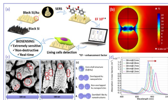
Fig. 3. (a, c) Design of a bSi-based gold-sputtered SERS-active substrate for the detection of trace molecule concentration and living cells. (b, d) FEM simulation results proving high signal enhancement factor due to the local surface plasmon resonance.
