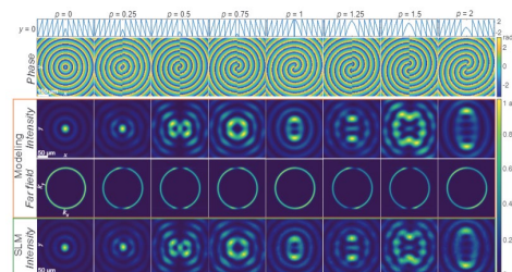
Fig. 3. Intensity patterns of non-diffracting beams as a function of the spatial displacement between two halves of axicon masks. The displacement p is given in steps of quarter period. The phase period r_0 = 80 \mu\text{m} and the Bessel beam cone half-angle \theta_c = 0.74^\circ . Bottom rows depict intensity distribution of experimentally generated beams.
