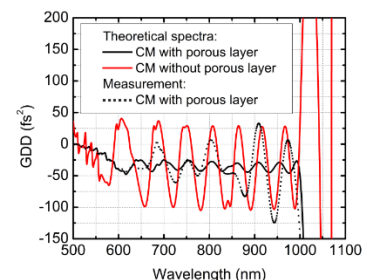
Fig. 12. Theoretical GDD spectra of two CM designs: with (black line) and without (red line) porous top layer. GDD measurement of deposited CM with porous layer is also depicted (black dots).
