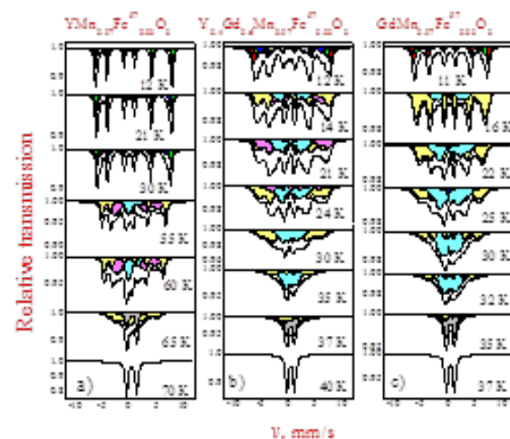
Fig. 2. (a) Mössbauer spectra of \text{YMn}_{0.97}\text{Fe}_{0.03}\text{O}_3 , (b) \text{Y}_{0.4}\text{Gd}_{0.6}\text{Mn}_{0.97}\text{Fe}_{0.03}\text{O}_3 and (c) \text{GdMn}_{0.97}\text{Fe}_{0.03}\text{O}_3 (c) at indicated temperatures.
