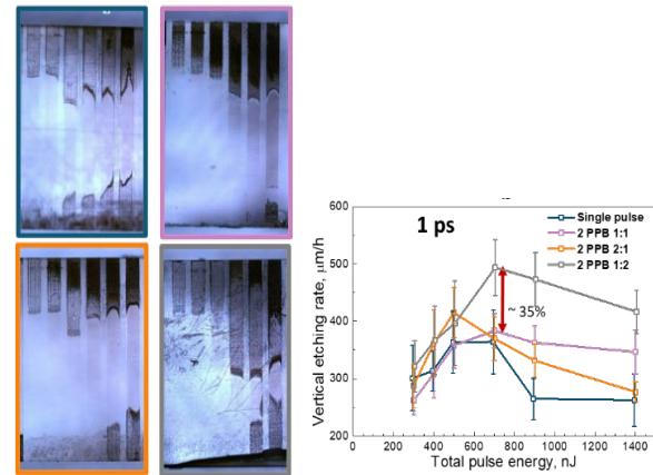
Fig. 16. The ER dependence on the pulse energy for vertical structures etched from the top surface in 10M KOH for 2 hours. The modifications were inscribed through the whole sample thickness. Dark areas from the top and bottom show the etched material. Laser pulse duration is 1 ps. The z-step distance was set to 5 \mu\text{m} . The colour border of the microscope pictures corresponds to the curve colour on the graphs. The error bar shows the standard deviation from the averaged value.
