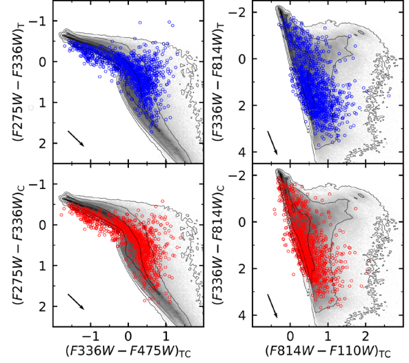
Fig. 1. Colour-colour diagrams show star cluster photometry results: (upper panels, blue dots) total (T) aperture photometry; (bottom panels, red dots) colour (C) aperture photometry. Distributions of star cluster models with masses from 10^2 to 10^5 M_{\odot} are plotted in the background (gray density contours). Colour indices indicated on the X-axis are constructed from T magnitudes in upper panels and C magnitudes in bottom panels. Arrows in the lower-left corners of panels indicate the extinction vectors of A_V = 1 , assuming the standard Milky Way extinction law.
