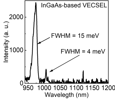
Figure 3.34: Lasing spectra of the InGaAs-based VECSEL designed for emission at 976 nm.
